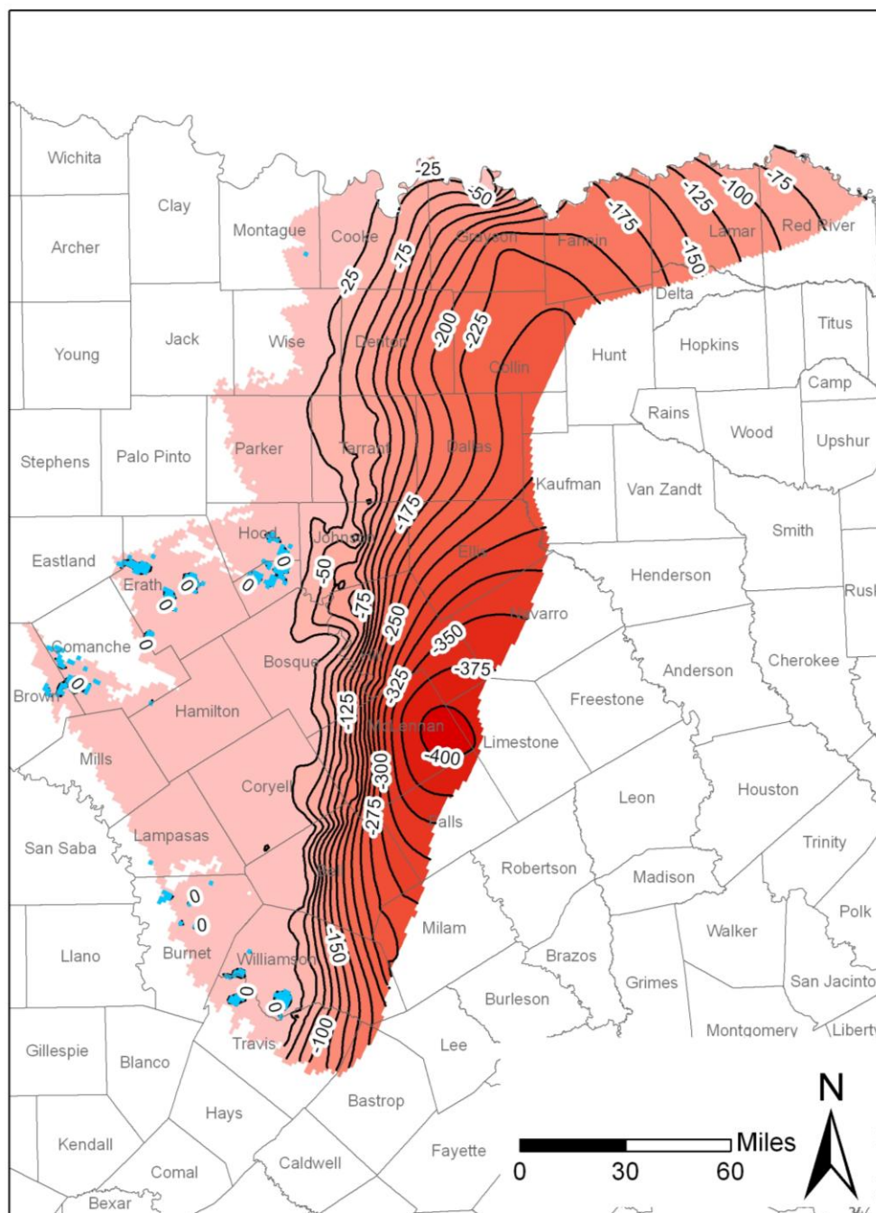
Figure 14. Changes in water levels after 50 years using the specified pumpage in layer 4 (Glen Rose Formation). Water level changes are in feet. Contour interval is 25 feet. Decreases in water levels (drawdowns) are shown in red. Increases in water levels are shown in blue. No cells converted to dry in layer 4.
