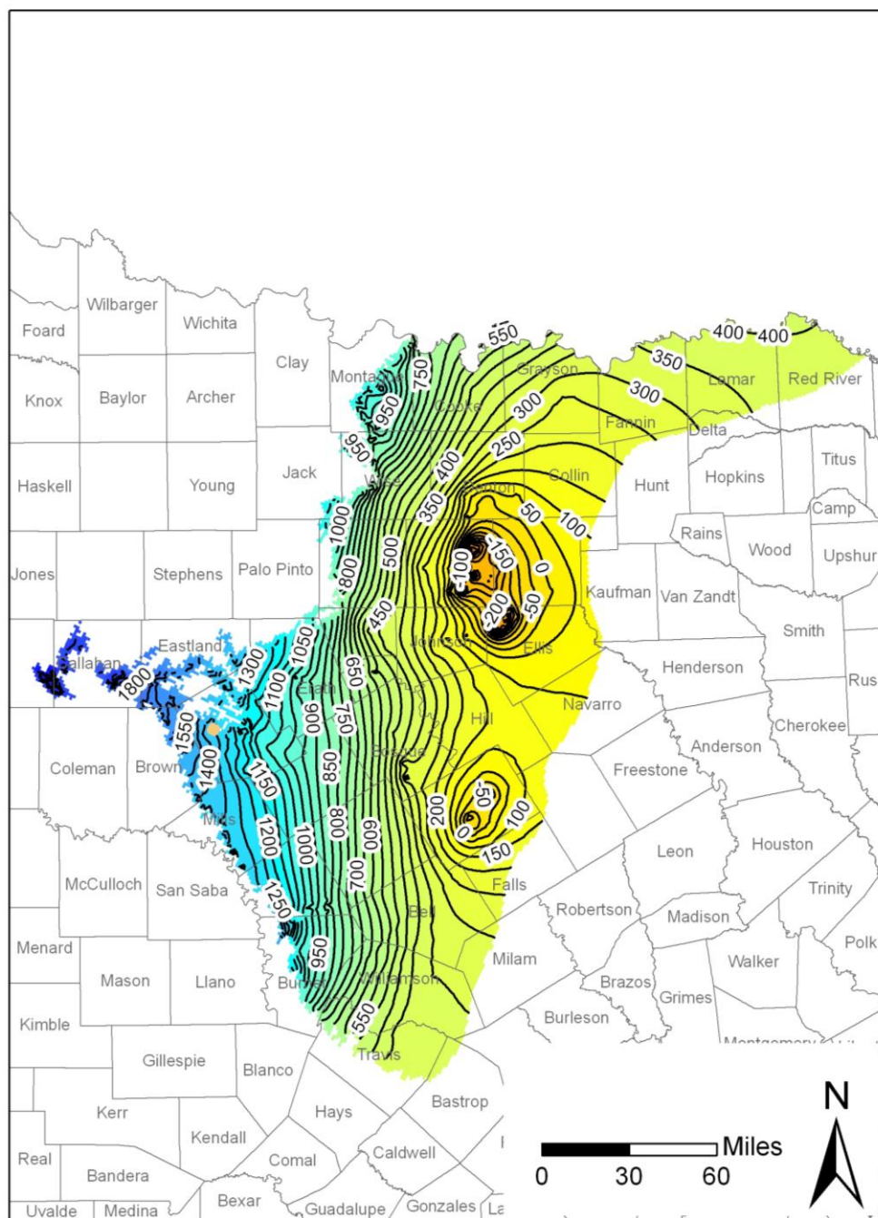
Figure 6. Initial water level elevations for the predictive model run in layer 7 (Hosston Aquifer) of the groundwater availability model for the northern part of the Trinity Aquifer System. Water level elevations are in feet above mean sea level. Contour interval is 50 feet. A dry cell, shown in tan, is located in Comanche County.
