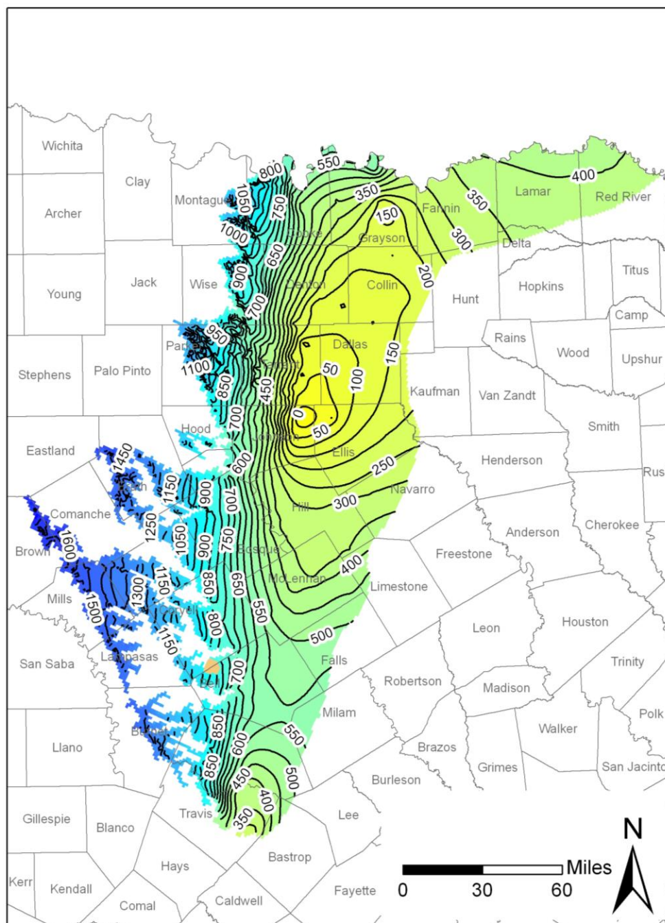
Figure 3. Initial water level elevations for the predictive model run in layer 3 (Paluxy Aquifer) of the groundwater availability model for the northern part of the Trinity Aquifer System. Water level elevations are in feet above mean sea level. Contour interval is 50 feet. Cells that converted to dry are shown in tan and are located in the vicinity of the Coryell-Bell county line.
