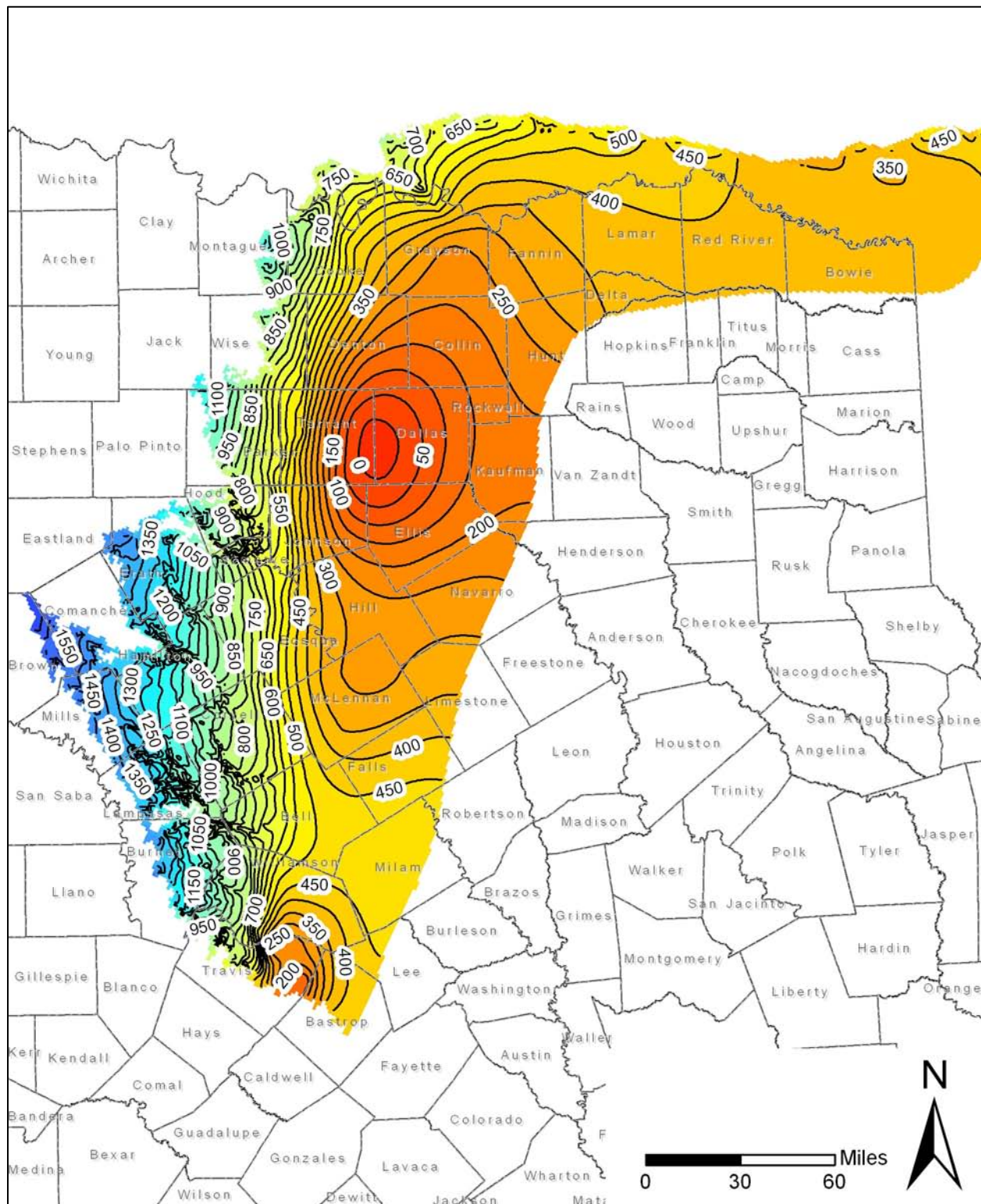
Figure 3. Initial water level elevations for the predictive model run in layer 4 (Glen Rose Formation) of the groundwater availability model for northern part of the Trinity Aquifer. Water level elevations are in feet above mean sea level. Contour interval is 50 feet.
