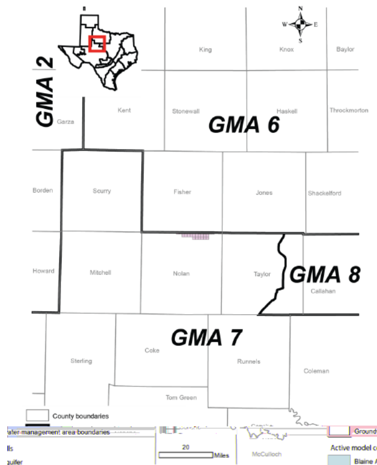
Figure 1. Location of Blaine Aquifer in GMA 7
