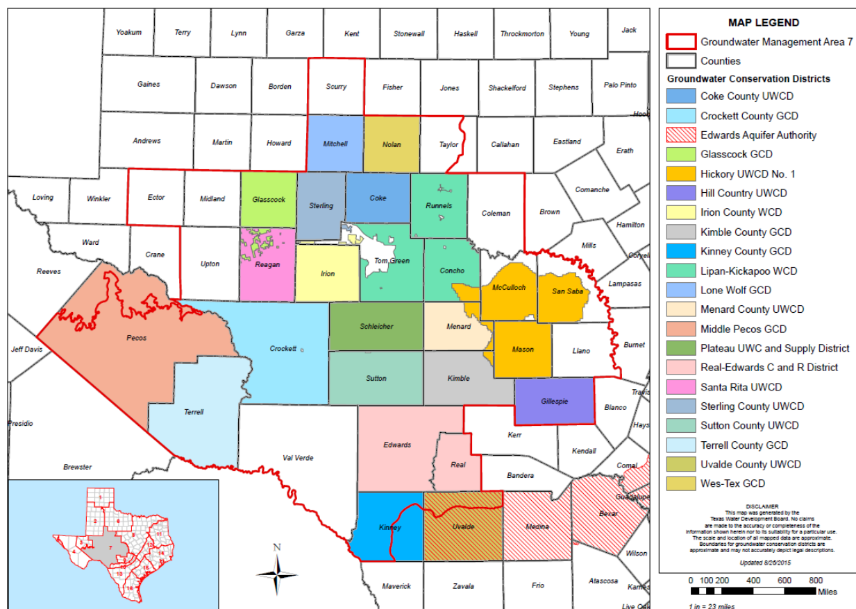
Figure 1. Groundwater Conservation Districts in Groundwater Management Area 7
